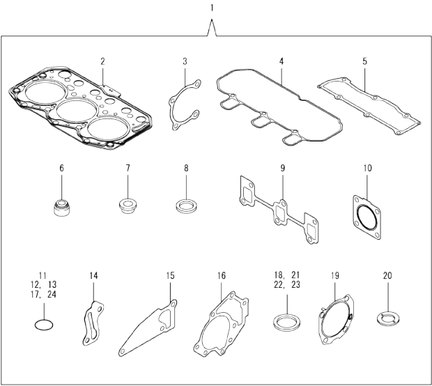
Fig.20. GASKET SET
