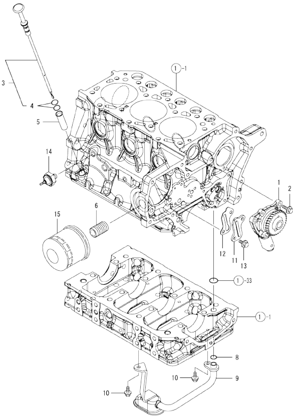
Fig.9. LUB.OIL SYSTEM
