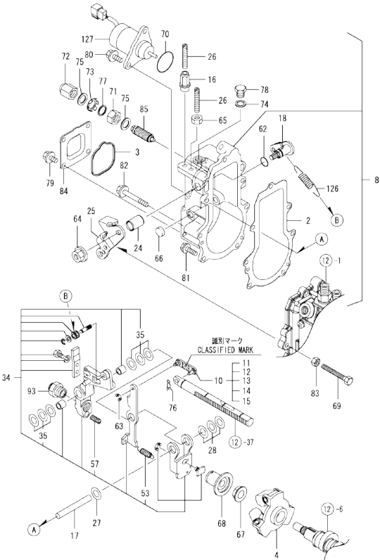
Fig.13. GOVERNOR
