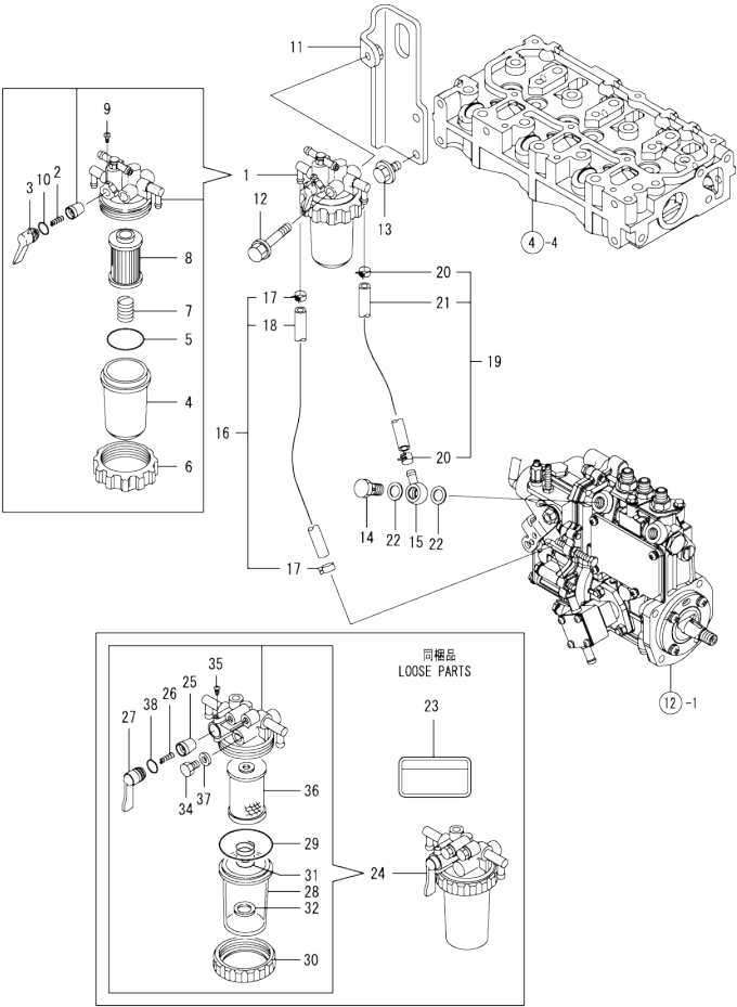
Fig.15. FUEL LINE
